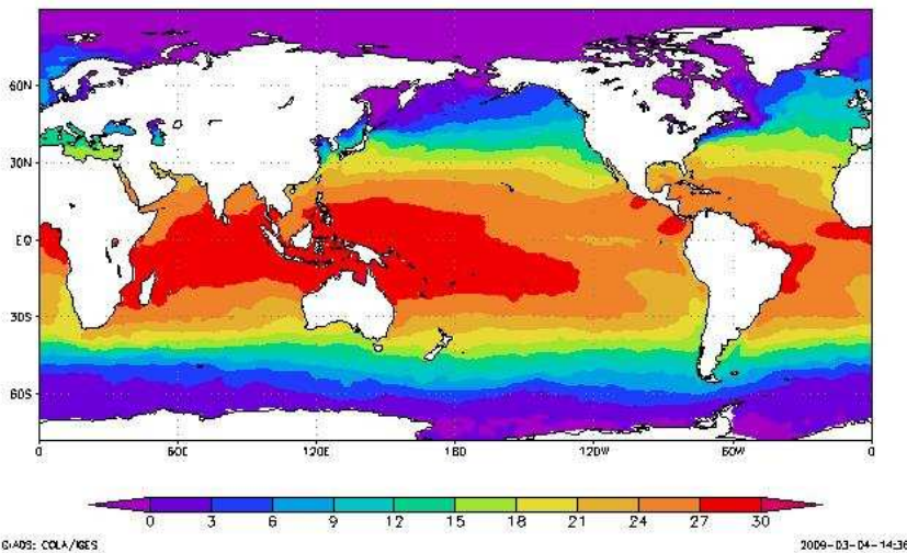
(c) Calculation by the model
