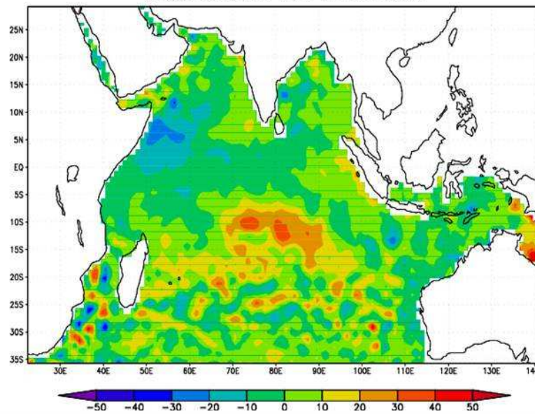
Slobs deviation from annual state
