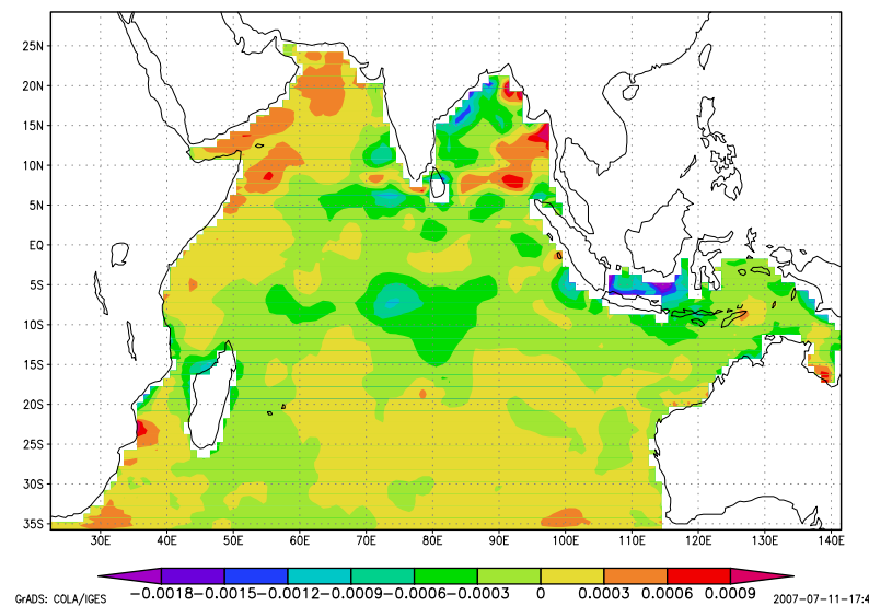
(b) Calculation with assimilation for \alpha = 10^5
