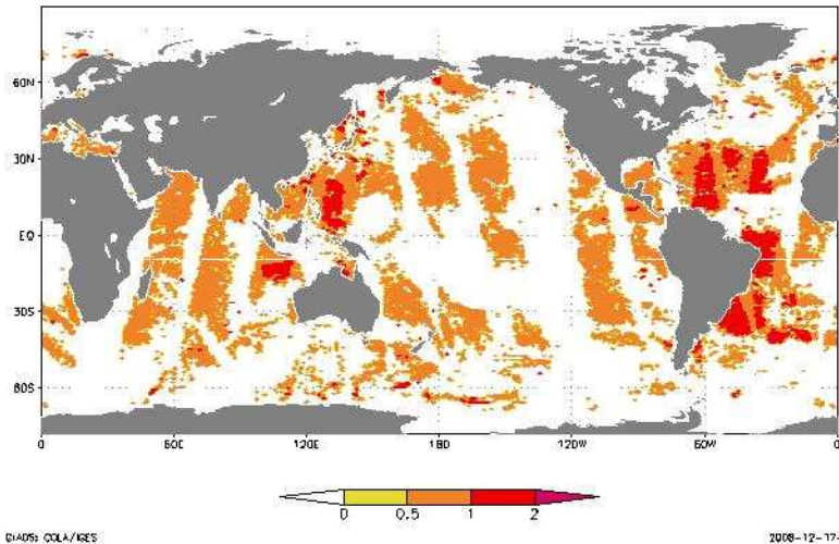
(a) Number of observation of SST (accumulated for 6 hours)
