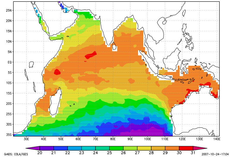
(b) Observation of SST 3 months and 3 days
