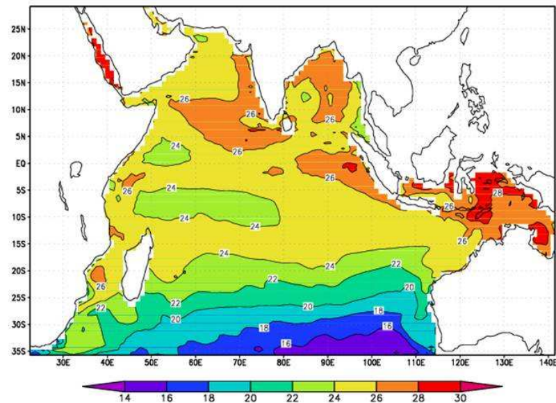
Tem50m 10d with assim
