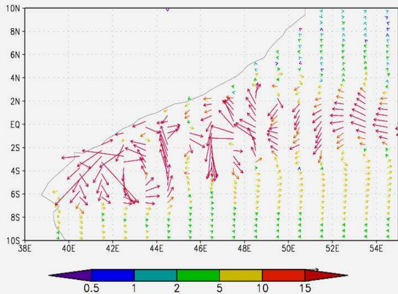
Vel difference between assim. and noassim
