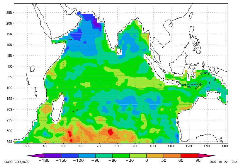
(b) Climatic mean heat flux
